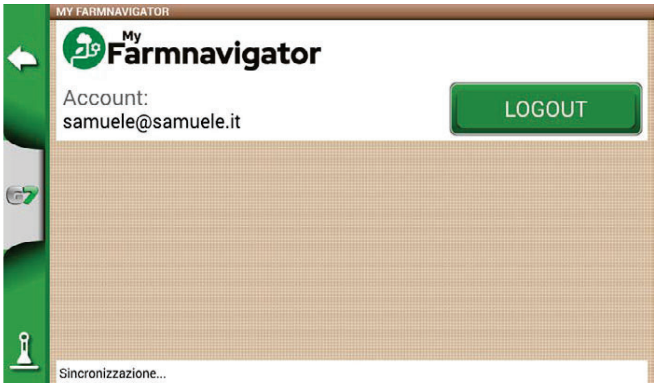
Figura 2.5.b - Login MyFarmnavigator
