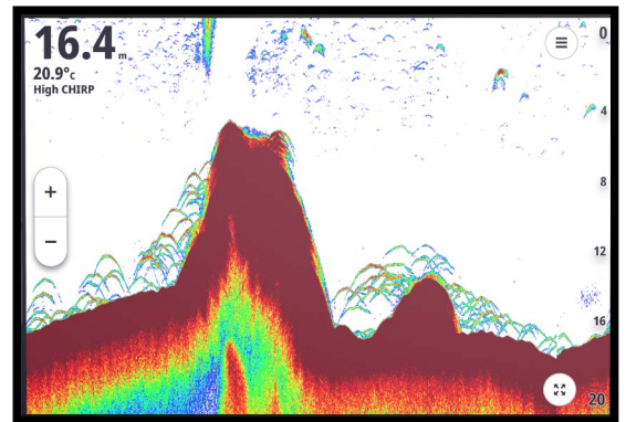
CHIRP sonar displays amazing detail and target separation
